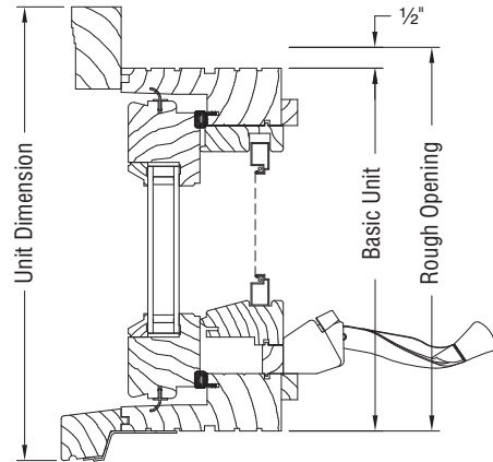
HEAD/SILL SECTION
