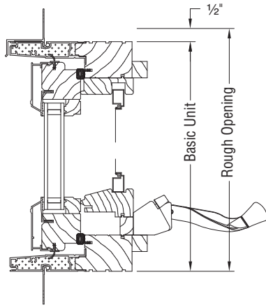
HEAD/SILL SECTION
