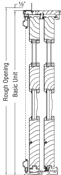
HEAD/SILL SECTION
