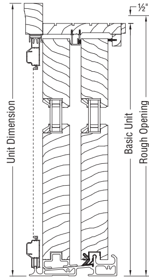
HEAD/SILL SECTION
