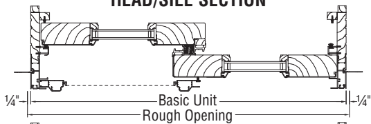
HEAD/SILL SECTION
