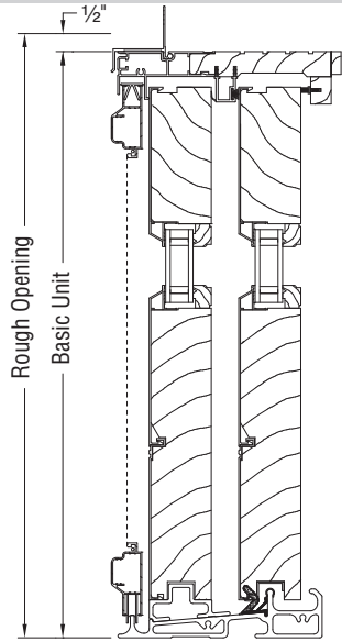
HEAD/SILL SECTION
