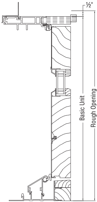
HEAD/SILL SECTION
