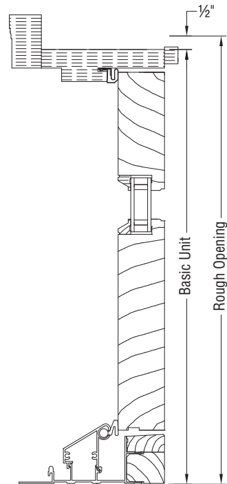
HEAD/SILL SECTION
