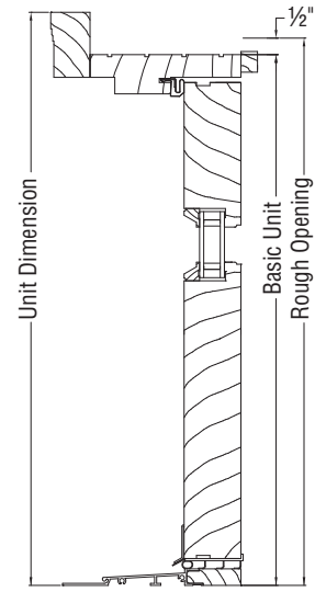
HEAD/SILL SECTION
