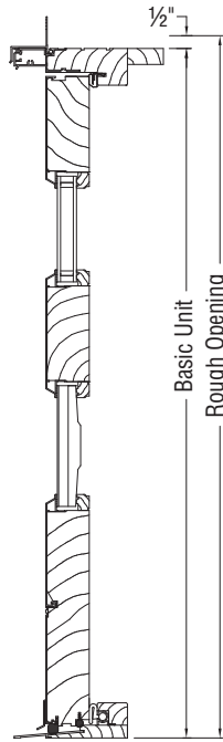
HEAD/SILL SECTION
