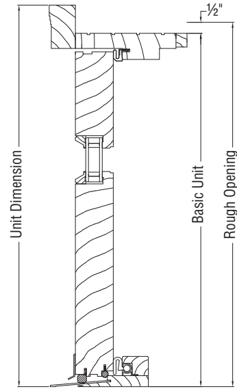
HEAD/SILL SECTION
