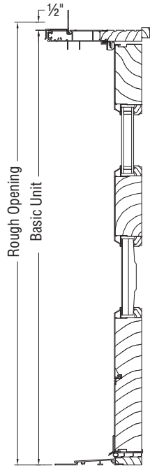
HEAD/SILL SECTION
