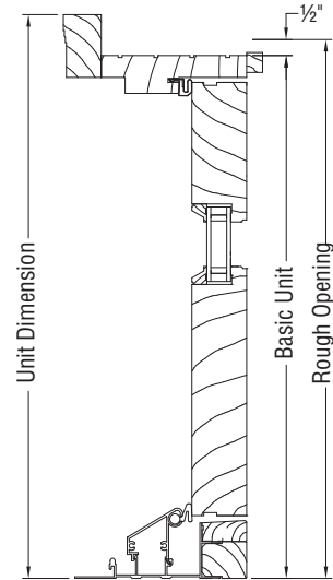
HEAD/SILL SECTION
