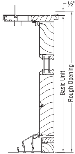
HEAD/SILL SECTION
