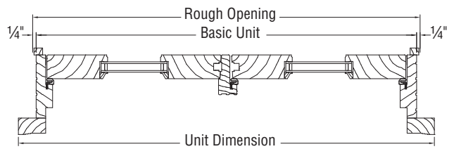
HEAD/SILL SECTION
