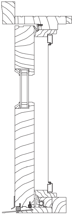
HEAD/SILL SECTION
