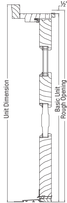
HEAD/SILL SECTION
