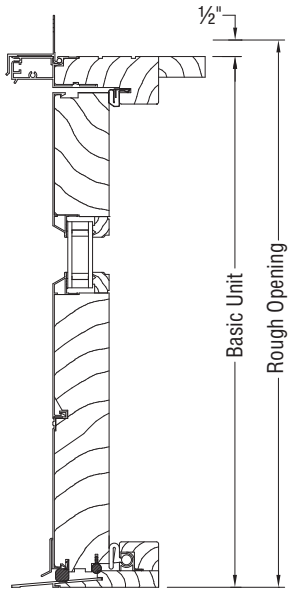
HEAD/SILL SECTION
