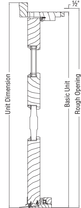
HEAD/SILL SECTION
