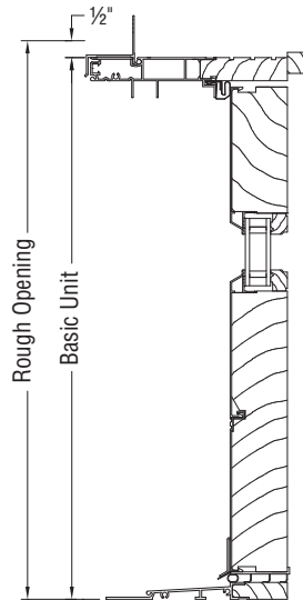
HEAD/SILL SECTION
